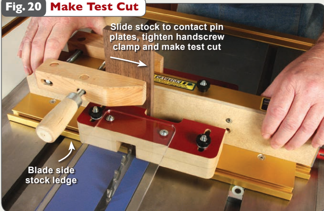
Fig. 20 Make Test Cut
