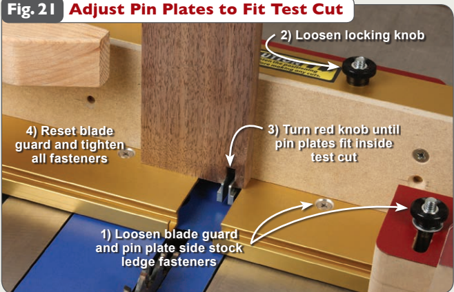
Fig. 21 Adjust Pin Plates to Fit Test Cut
