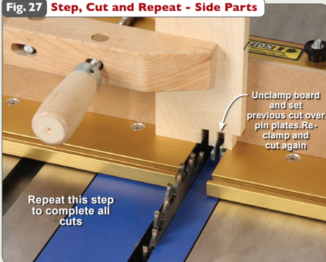
Fig. 27 Step, Cut and Repeat - Side Parts
