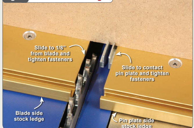
Fig. 17 Position Stock Ledges
