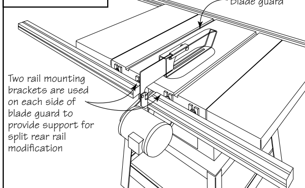
FIG. 26 Rear rail modification
