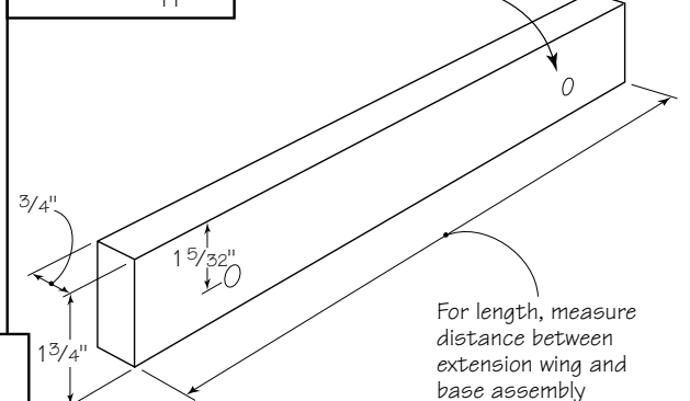
FIG. 28 Table board support
